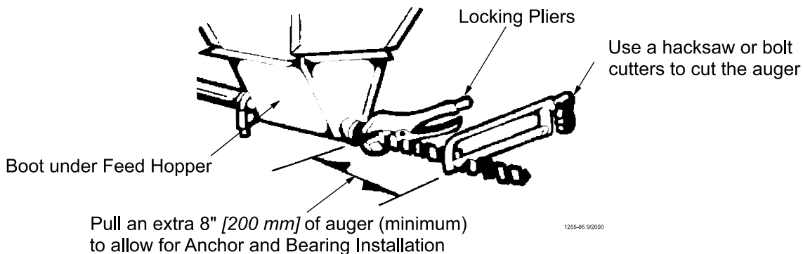
Figure 56. Cut Auger
