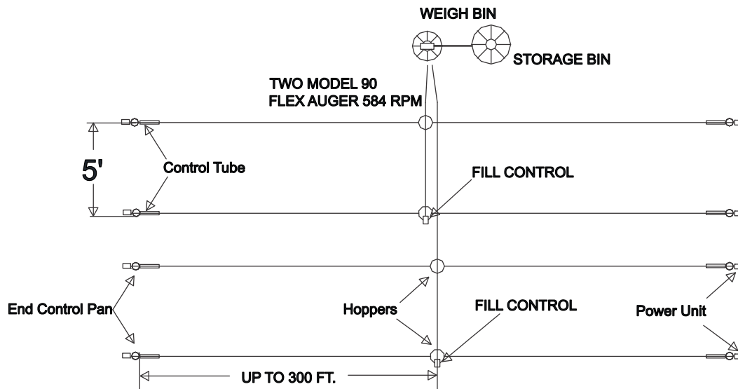
Figure 1. Planning the system
