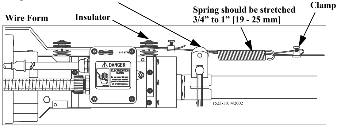
Figure 47. Cable hook up at Power Unit.
