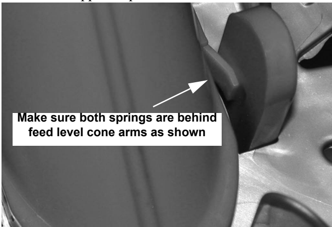
Figure 29. Support Cap Installation
