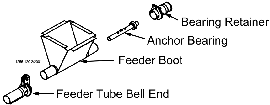
Figure 50. Installing the Feeder Boot
