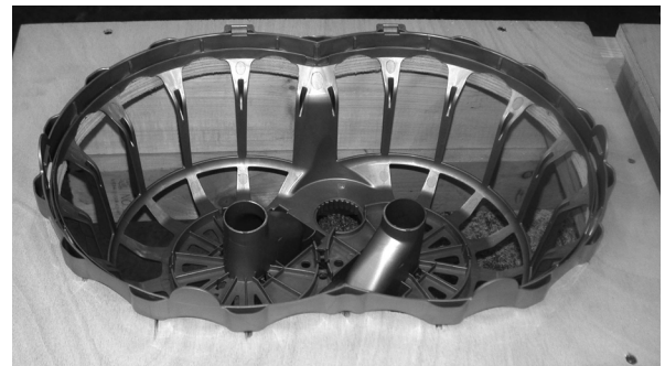
Figure 31. Place Grill into Assembly Fixture
