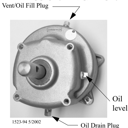
Figure 65. Gearhead Maintenance
