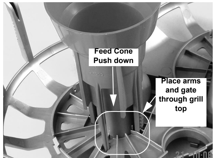
Figure 32. Install feed cones
