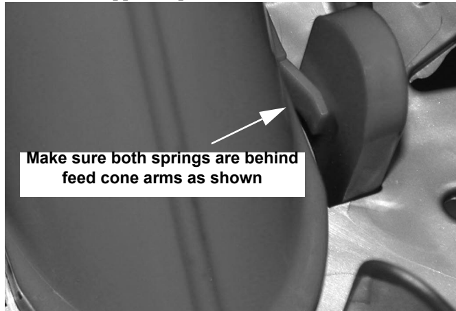
Figure 38. Support Cap Installation
