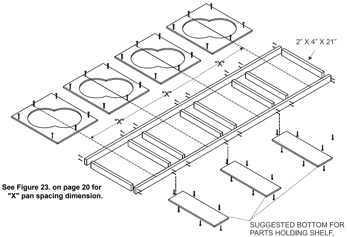
Figure 22. Feeder Pan and Tube Assembly Fixture Construction
