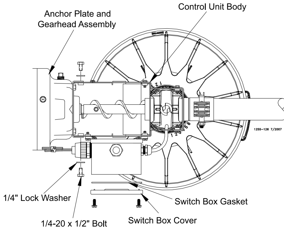
Figure 53. Attaching the Anchor Plate and Gearhead Assembly to the Control Unit Body
