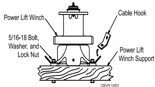
Figure 5. Assembling the Power Winch to the Rafters
