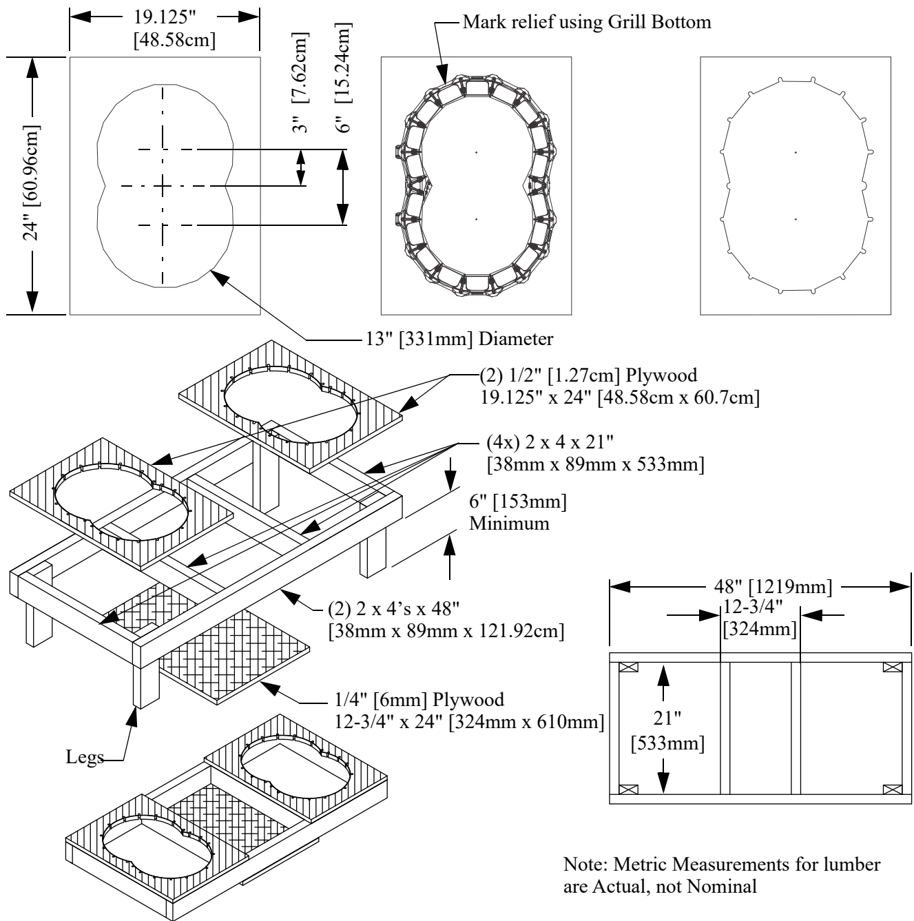
Figure 30. Feed Pan Assembly Box Construction
