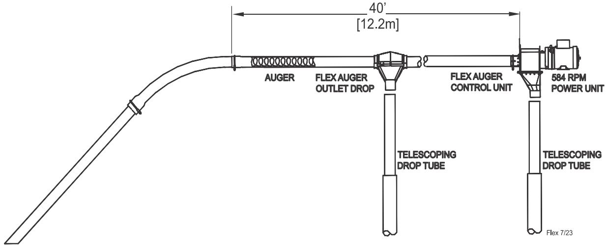
Sample FLEX-AUGER layout for reference only.
