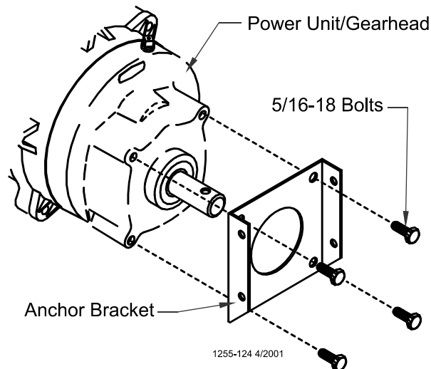
Figure 51. Assemble the Anchor Bracket to the Power Unit/Gearhead
