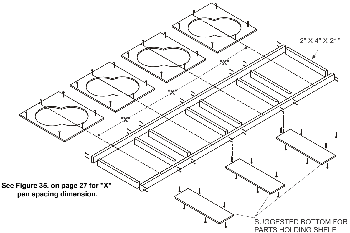
Figure 34. Feeder Pan and Tube Assembly Fixture Construction
