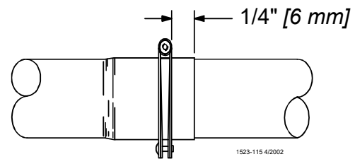
Figure 42. Clamp Installation
