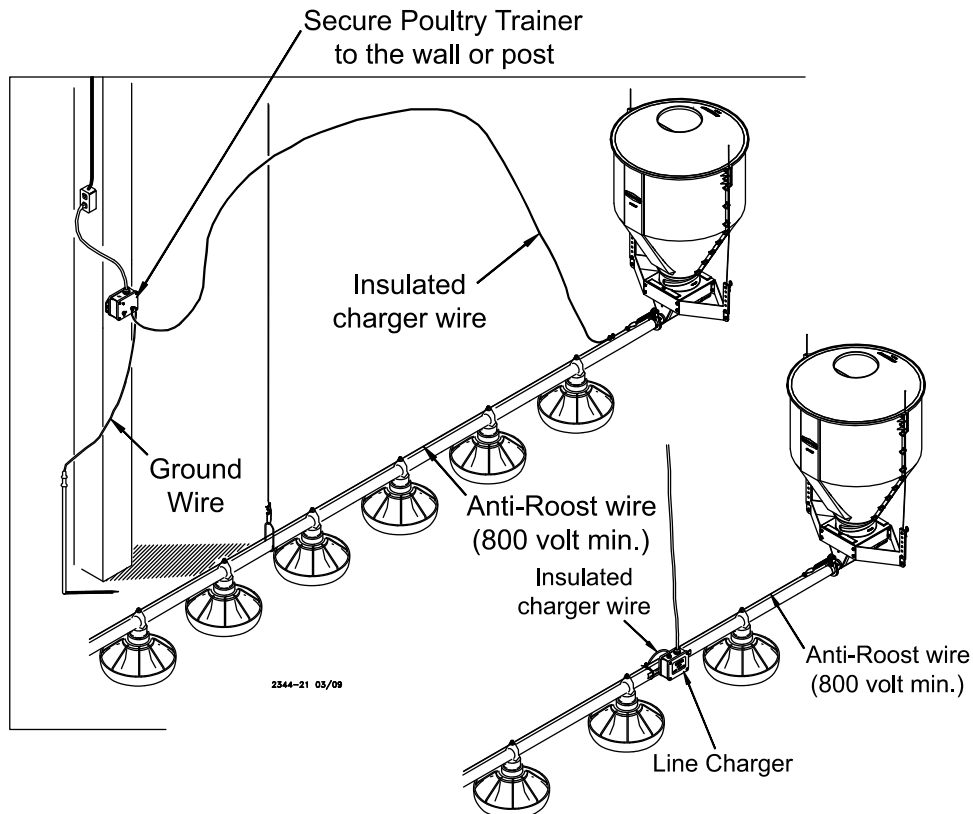
Figure 48. Poultry Trainer Installation
