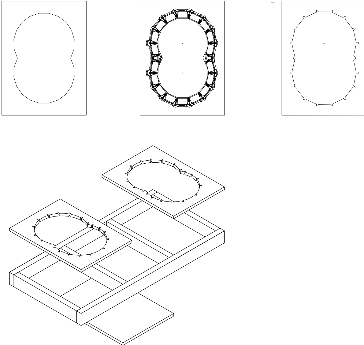
Figure 17. Feed Pan Assembly Box Construction
