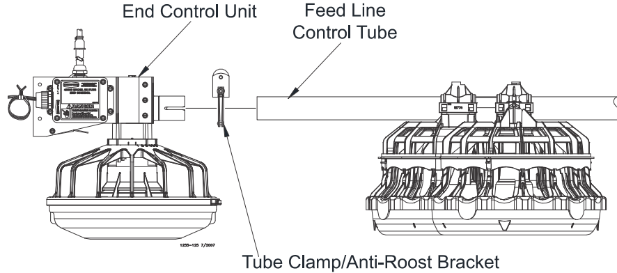
Figure 49. Connecting End Control Unit to the Feed Line Tube
