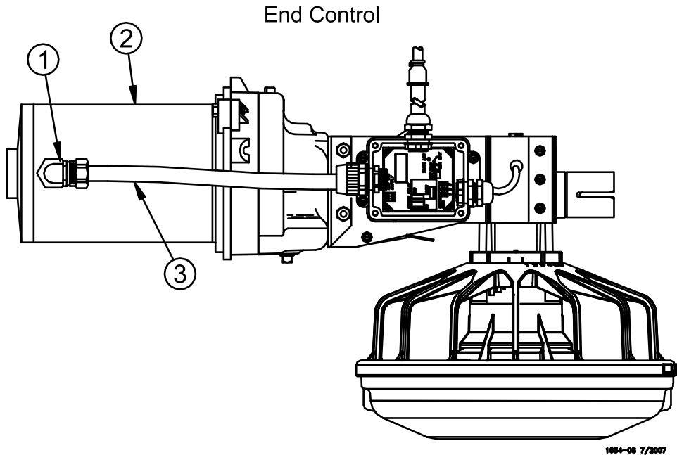
Figure 54. Wiring the Motor
