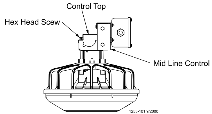
Figure 60. Mid-Line Control Installation
