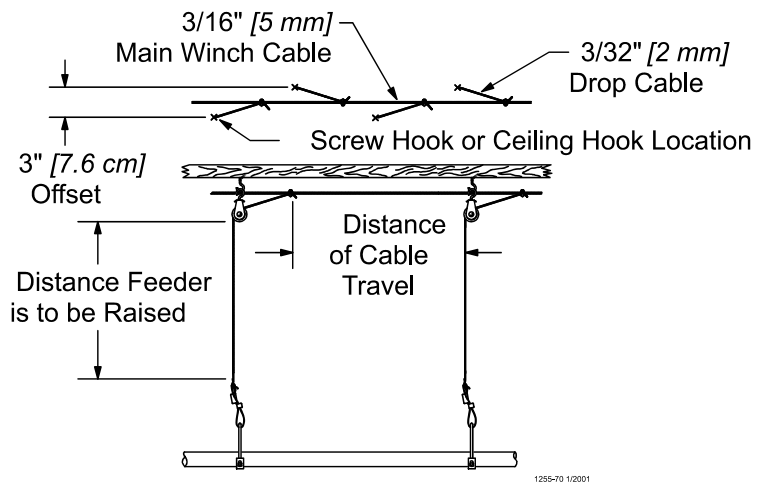
Figure 12. Drop Line Off Set Detail
