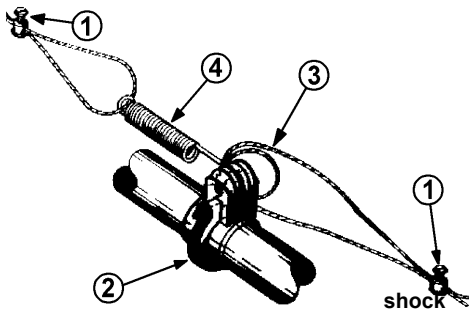
Figure 46. Anti-Roost Cable Mid-Line Connection
