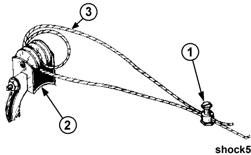
Figure 45. Anti-Roost Cable at the Hopper
