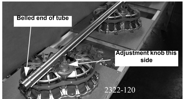
Figure 28. Height Ring Installation
