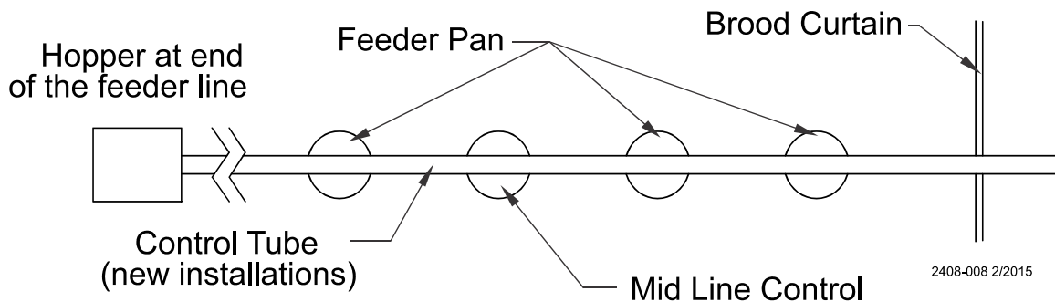
Figure 39. Mid-Line Control Location Diagram
