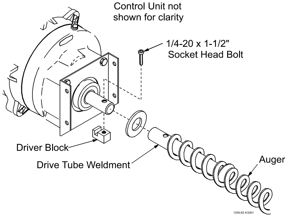
Figure 31. Auger Driver Components
