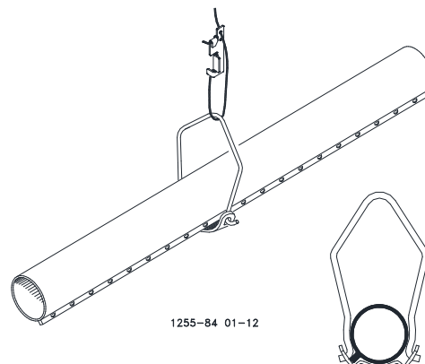
Figure 27. Hanger Installation
