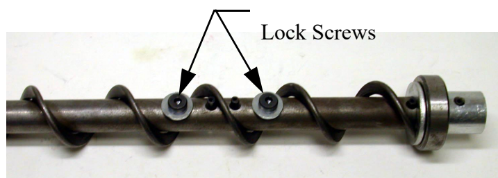
Figure 51. Auger and anchor Bearing Connection
