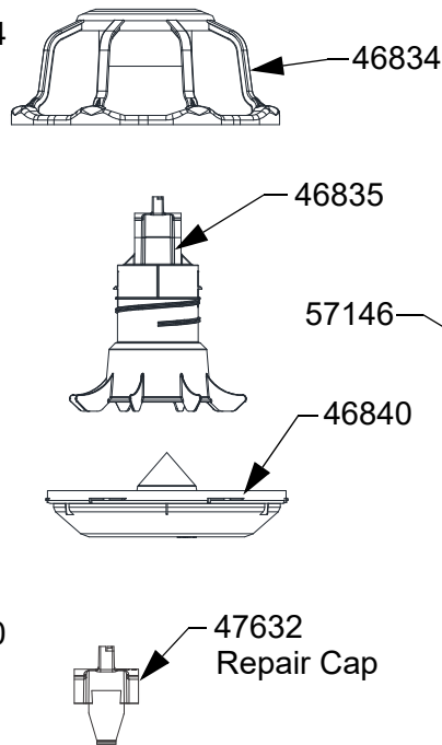
47675 FF Revolution® Feeder 8 Spoke Non-Window
