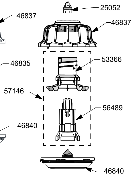
57144 FF Revolution® Feeder 12 Spoke w/Two Piece Top
