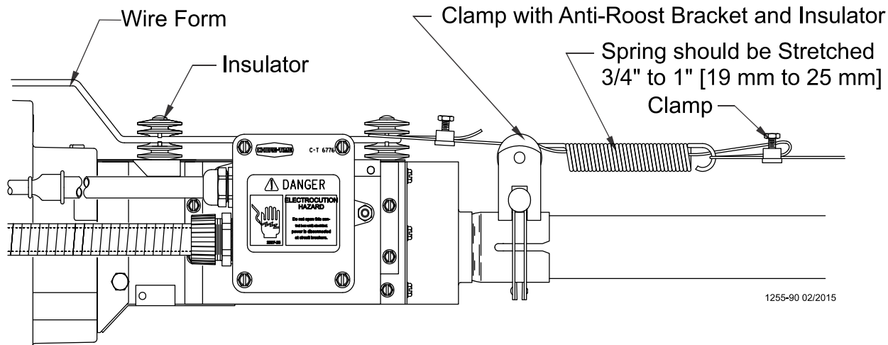
Figure 44. Anti-Roost Installation at the Control Unit
