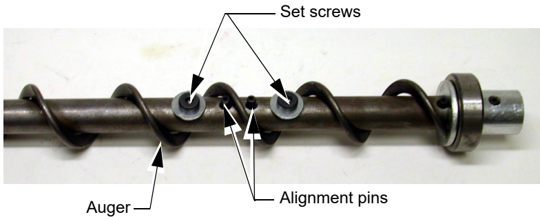
Figure 36. Auger and Anchor Bearing Connection
