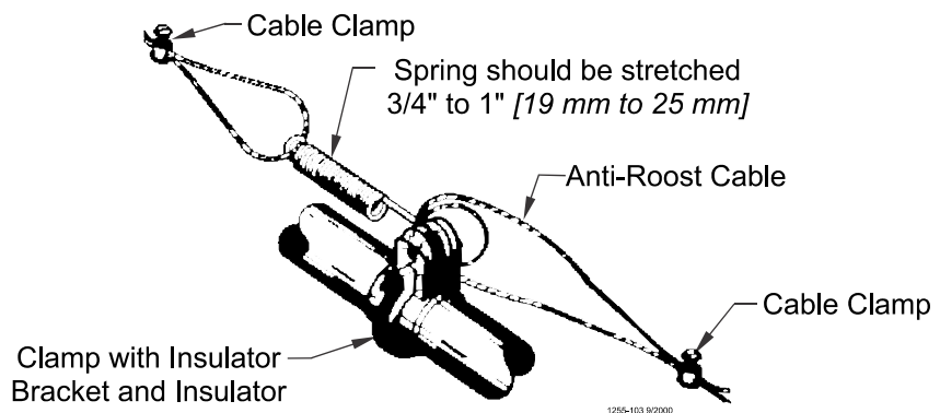
1255-103 9/2000 Figure 43. Anti-Roost Cable Mid-Line Connection
