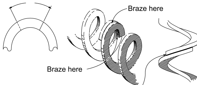
Figure 37. Auger Brazing
