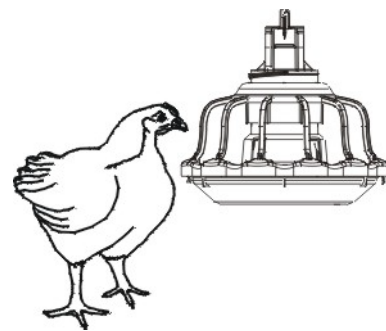
Figure 49. Feeder Pan Assembly height adjustment
