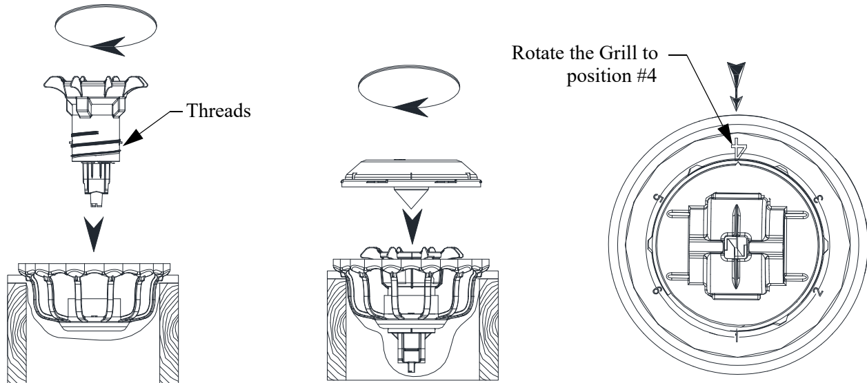
Figure 24. Pan Assembly Option 1
