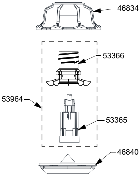
53368 FF Revolution® Feeder 8 Spoke w/Windows
