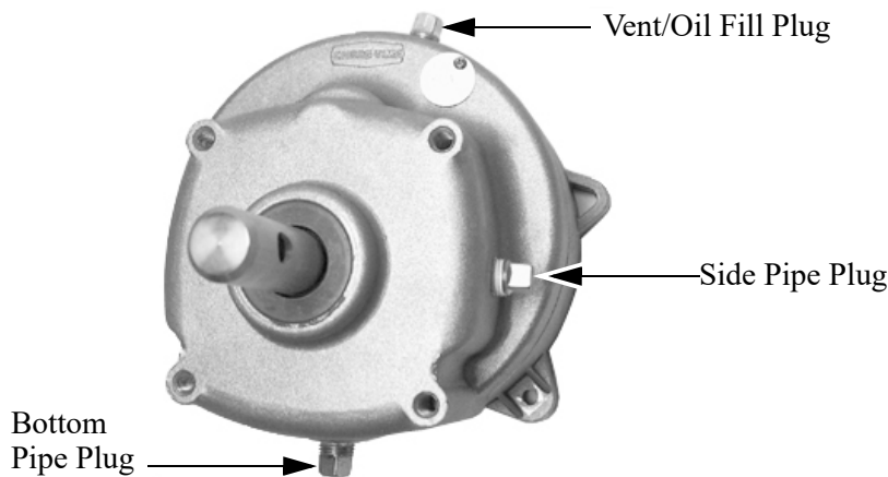
Figure 50. Gearhead Maintenance
