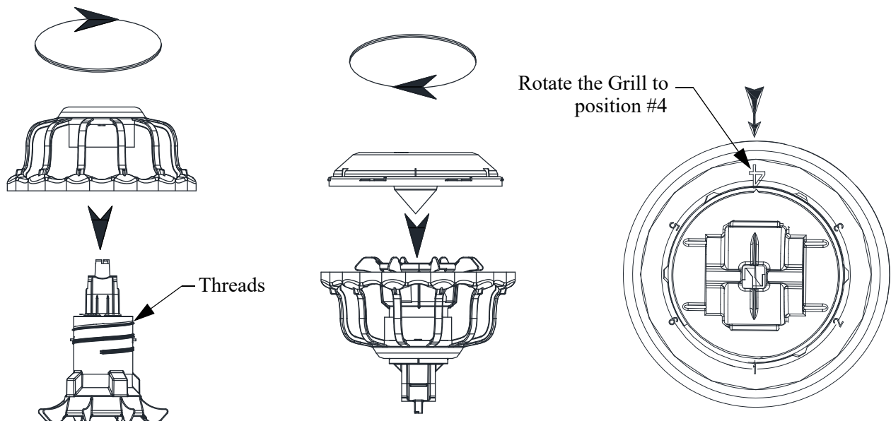
Figure 25. Pan assembly option 2
