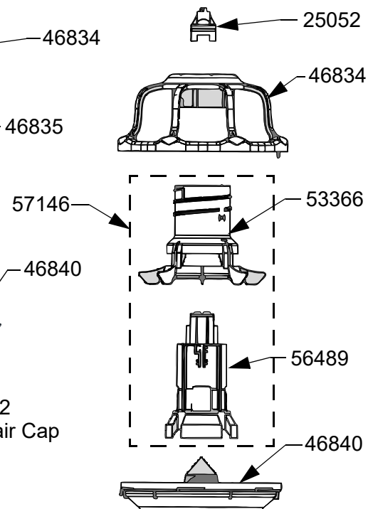
57145 FF Revolution® Feeder 8 Spoke w/Two Piece Top
