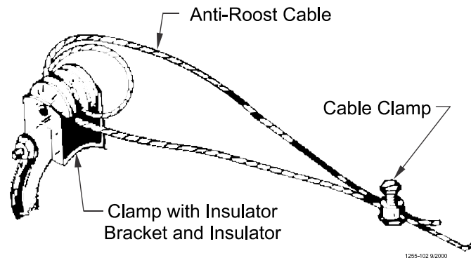
1255-102 9/2000 Figure 42. Anti-Roost Cable at the Hopper
