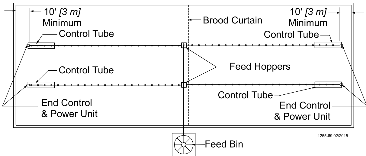
Figure 46. Component location diagram for systems over 400 feet [122 m]. (Top View).
