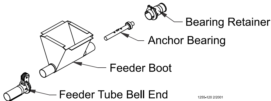
Figure 29. Installing the Feeder Boot
