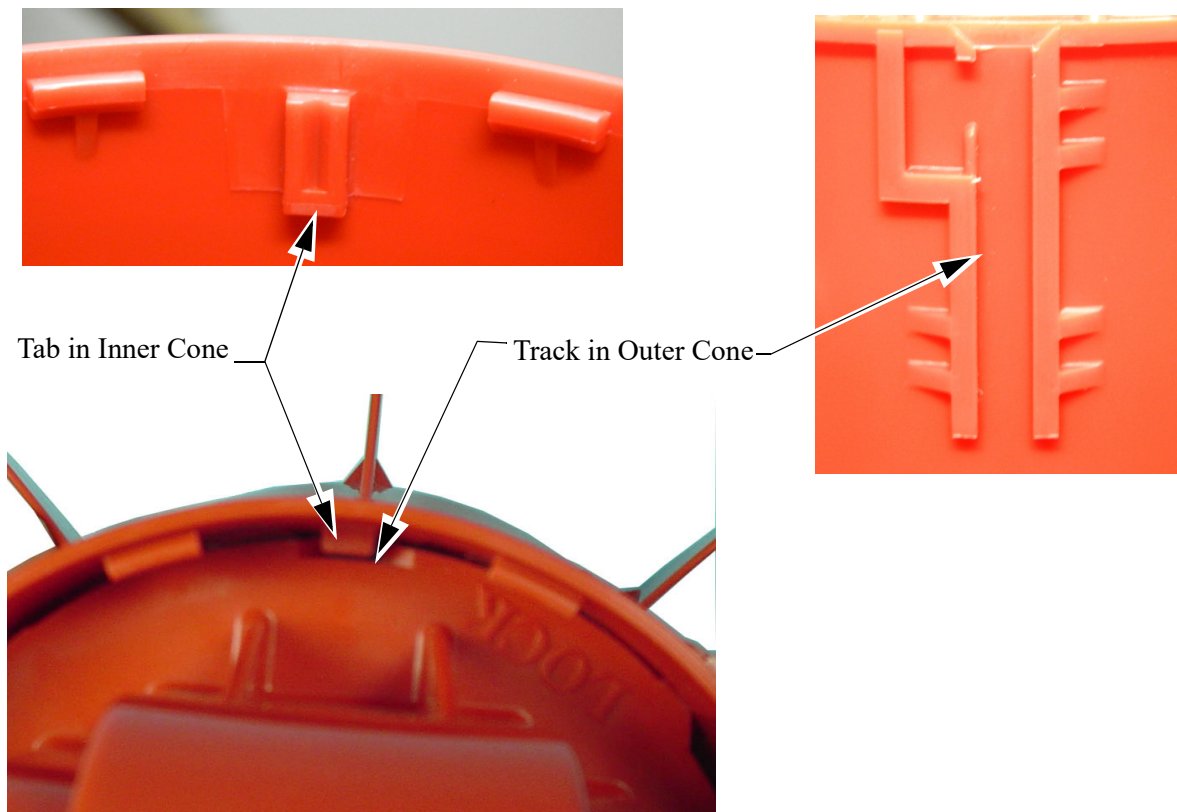
Figure 22. Tab and Track alignment
