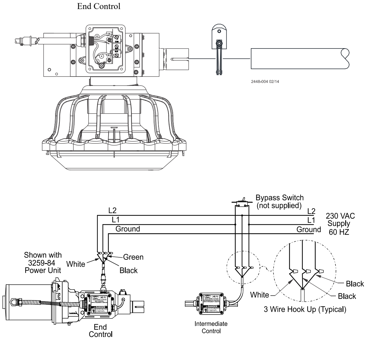
Figure 53. End Control Internal Wiring
