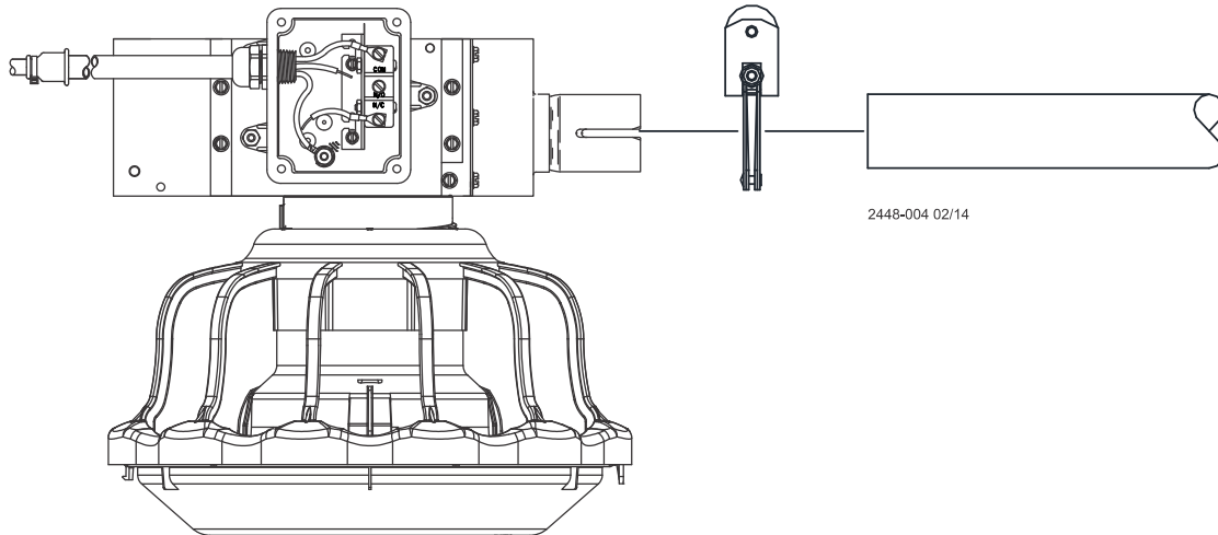
Figure 28. Connecting End Control Unit to the Feed Line Tube
