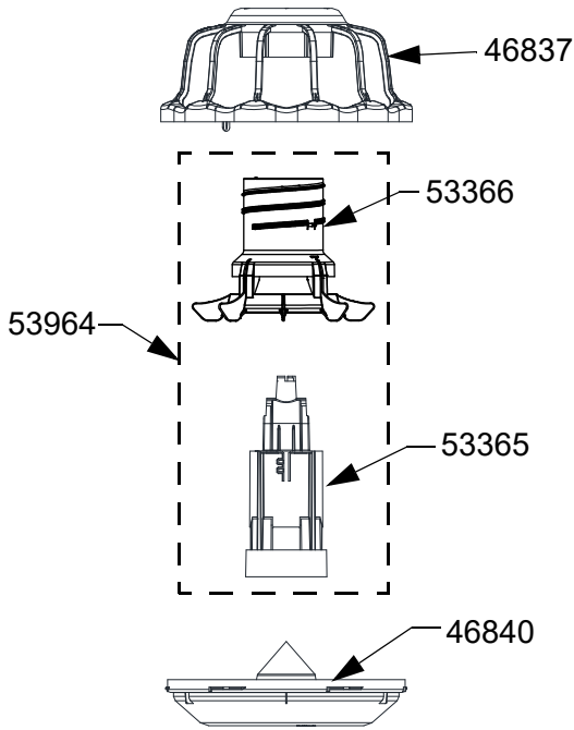
53367 FF Revolution® Feeder 12 Spoke w/Windows
