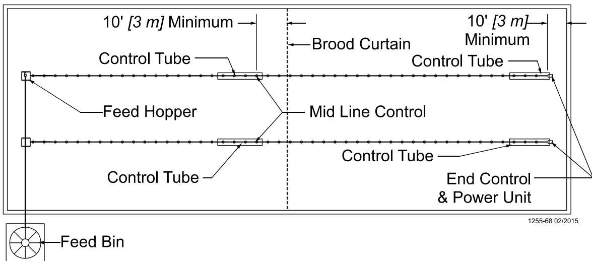
Figure 47. Component location diagram for systems up to 400 feet [122 m]. (Top View).
