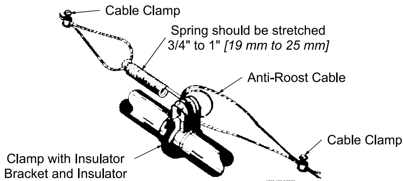
Figure 39. Anti-Roost Cable Intermediate Connection
