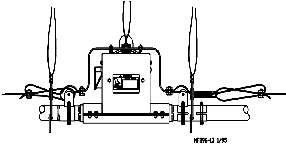
Figure 40. Anti-Roost Installation at the Control Unit
