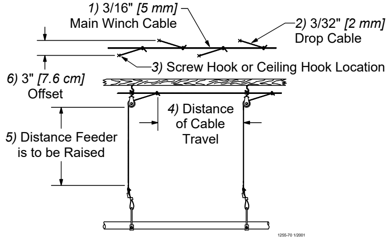
Figure 10. Drop Line Off Set Detail
