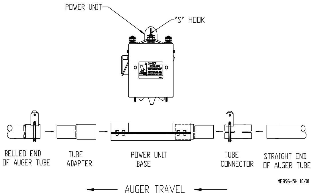
Figure 29. Power Unit Installation (View Standing outside the loop)
