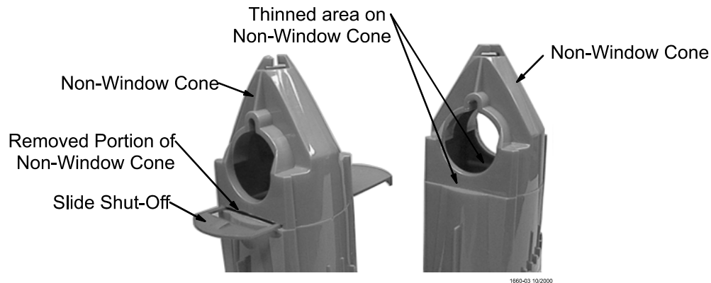
Figure 51. Optional Slide Shut-Off Assembly
