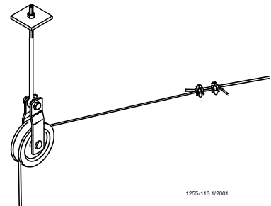
Figure 6. Full Line Suspension Kit
