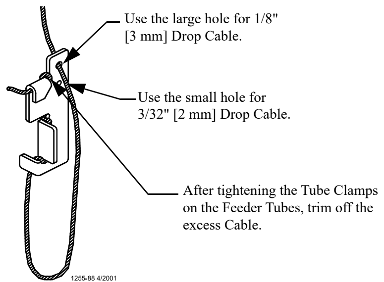
Figure 27. Cable Lock Threading
