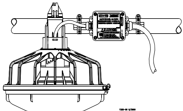
Figure 48. Installing the Sensor Plus Mid-Line Control
