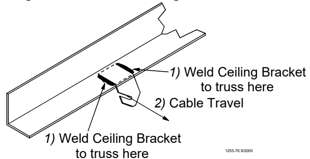
Figure 13. Welded Steel Truss Ceiling Bracket Installation
