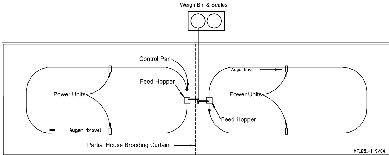
Figure 1. Planning the System
