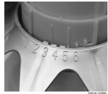
Figure 49. Feeder Pan Assembly adjustment
