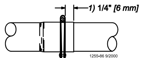
Figure 25. Clamp Installation
