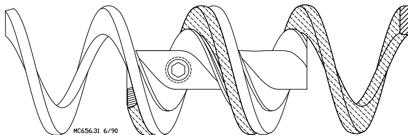
Figure 34. Auger Connector
