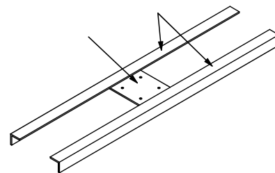
Figure 3. Optional Power Lift Winch support detail
