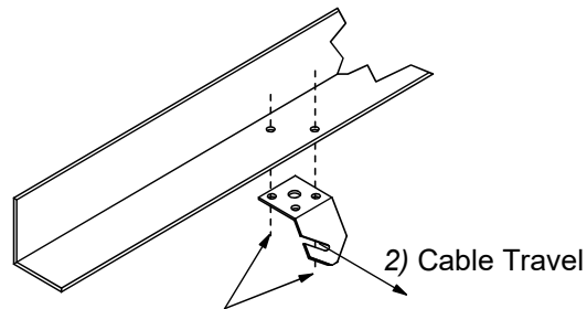
1) Secure Ceiling Hook to truss using self-drilling screws through opposite holes
