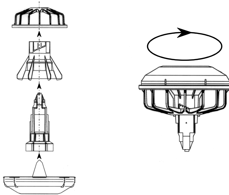
Figure 20. Assembling the Feeder Pan
