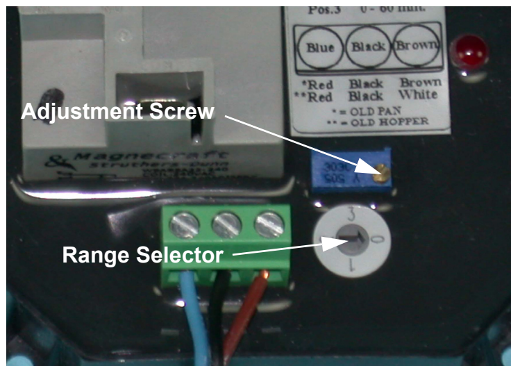
Figure 55. Adjusting the Sensor Plus Proximity Switch
