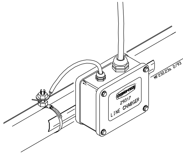
Figure 43. Line Charger Installation
