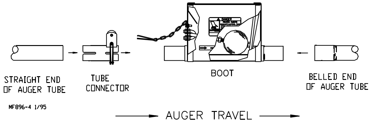
Figure 28. Boot components for Recommended Hopper Location (View Standing inside Loop)
