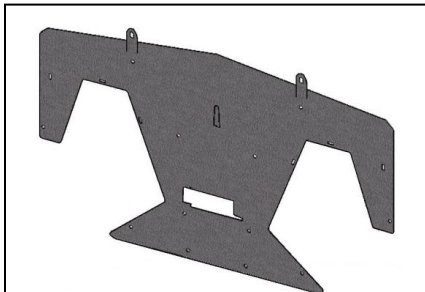
16550080B END PLATE CONTROL END 1 each
