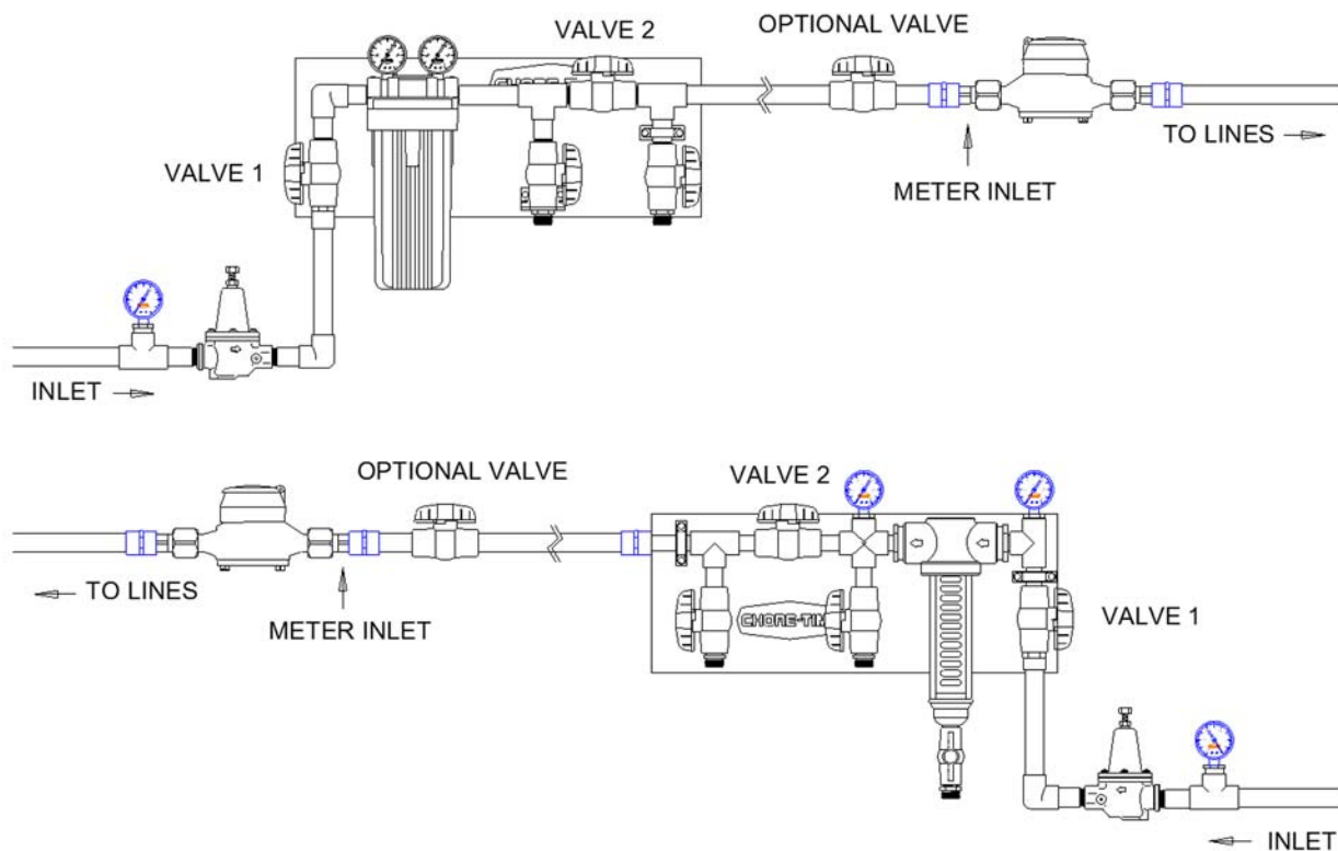
Figure 24. Water Meter Start Up
