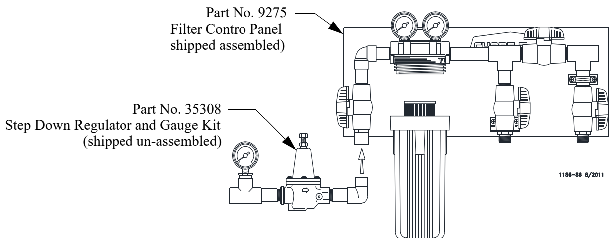
Figure 21. 9275 Control Panel
