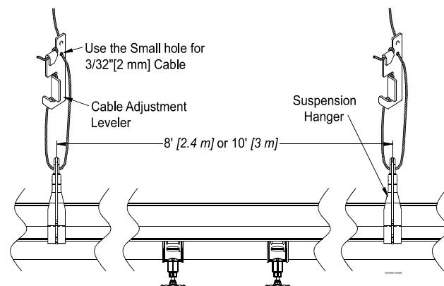
Figure 13. Suspension Hanger Location
