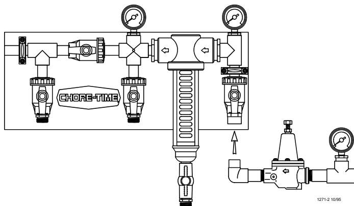
High Pressure Control Panel Part Number 36802-2
