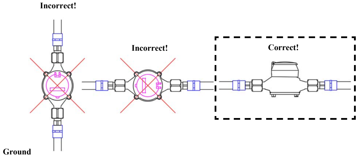
Figure 23. Water Meter Mounting
