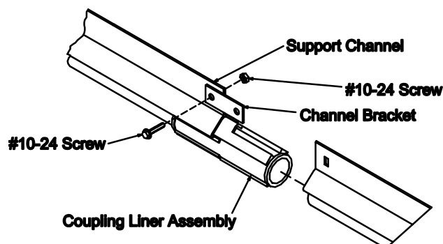
Figure 15. Securing the Water Line together Assembly Installation
