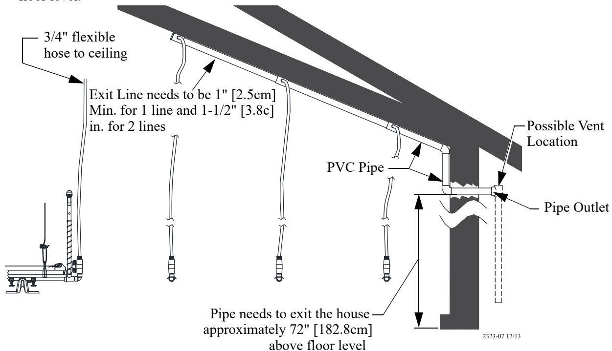
Figure 27. Anti-Roost Components
