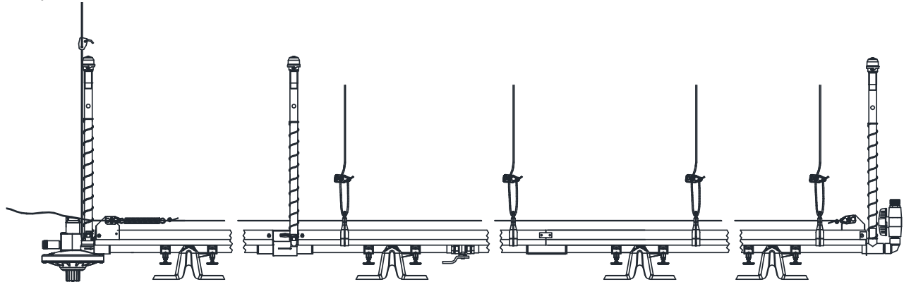
Figure 25. Regulator End Components
