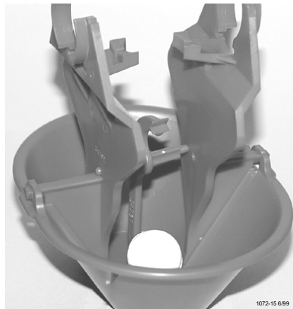
Figure 4. Pivot Arm Installation
