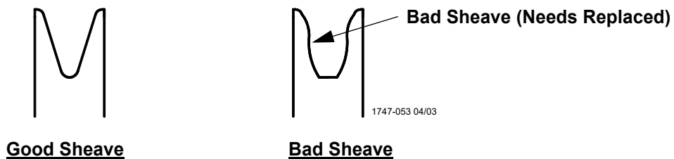
Figure 24. Sheave Condition
