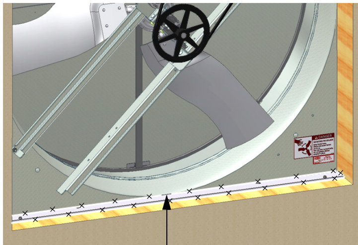
Shroud Drain Hole (Do not Caulk Drain Hole Shut!)
