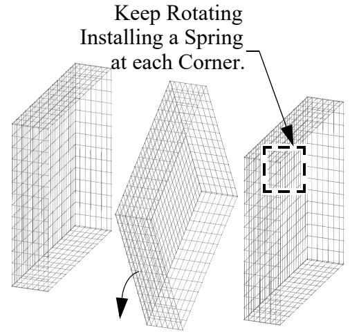
3. Rotate the Screen in the direction shown installing a Spring at a second corner. Repeat for remaining Corners.
