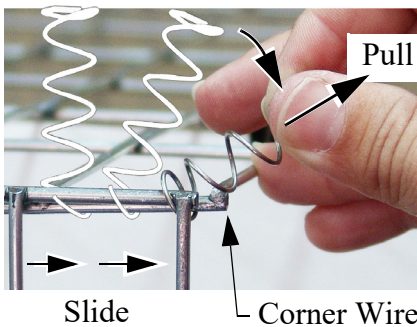
C) Slide and Pull Spring over Corner Panel Wire.
