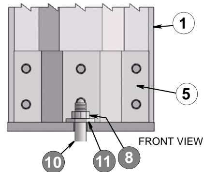
Figure 33a. Leg Anchor Weldment
