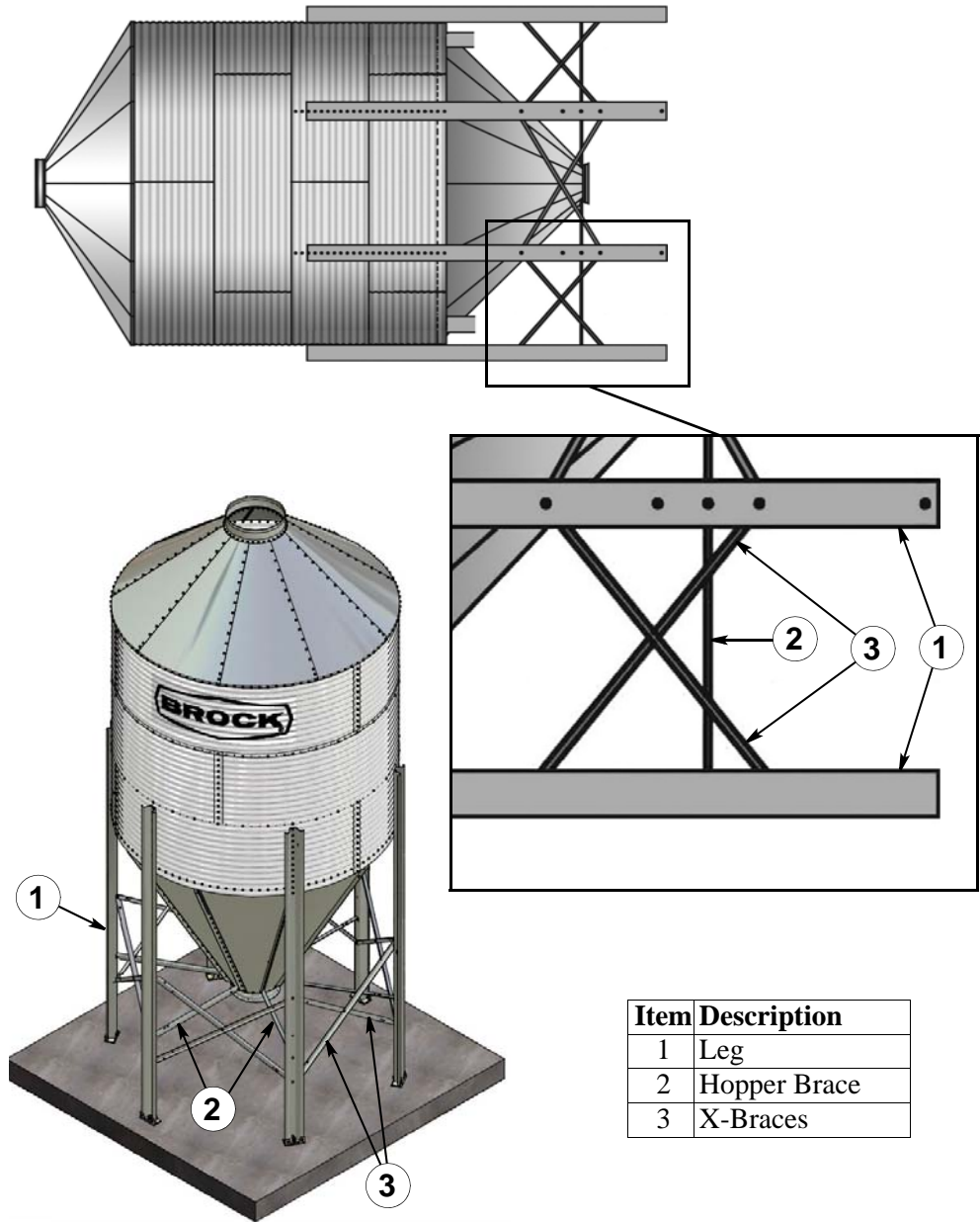
Figure 30. Brace Attachment
