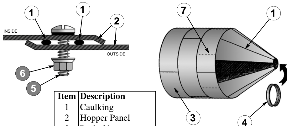
Figure 23. Hopper Collar
