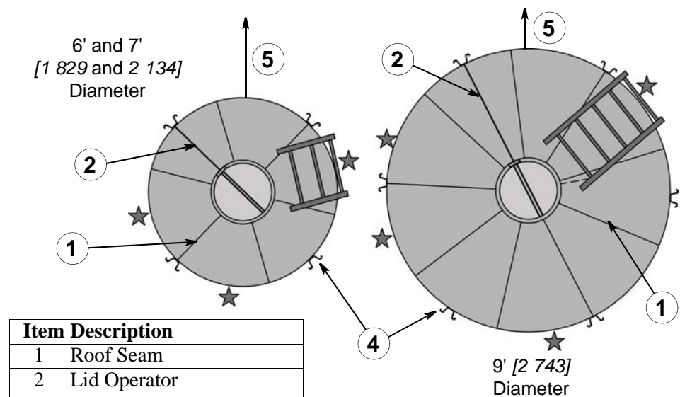
Figure 22. Possible Roof Ladder Locations
