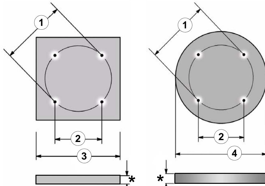
SQUARE FOUNDATION
