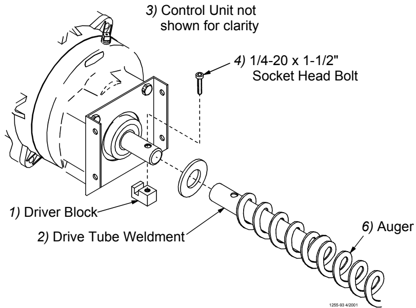
Figure 35. Auger Driver Components
