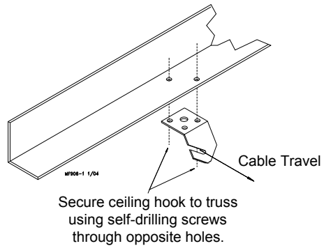
Figure 16. Wide Steel Truss Ceiling Installation
