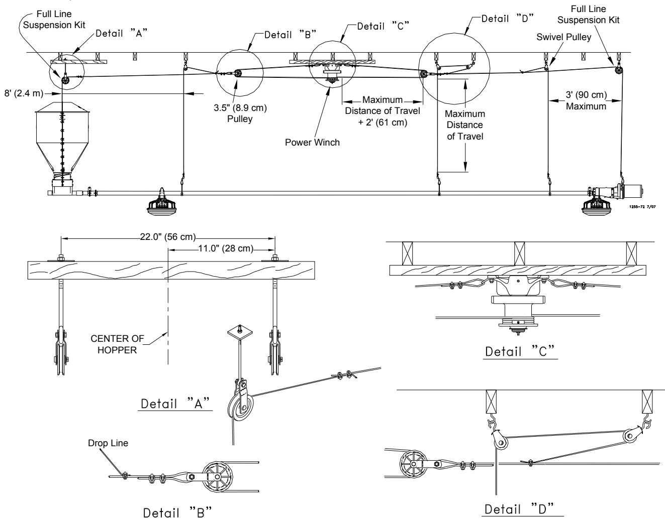
Figure 3. Suspension for systems over 350' [107 m]
