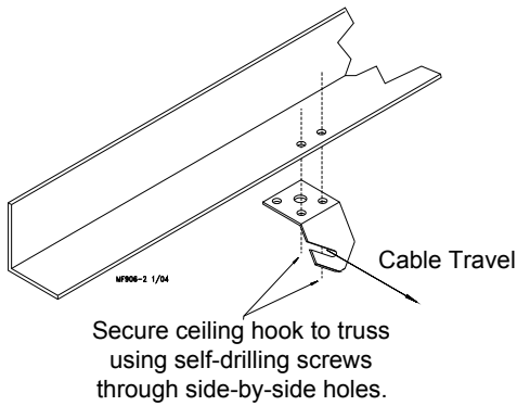
Figure 15. Narrow Steel Truss Installations
