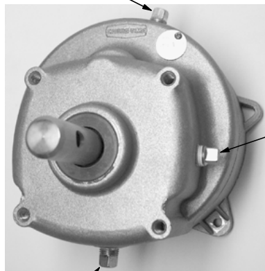
Figure 58. Gearhead Maintenance
