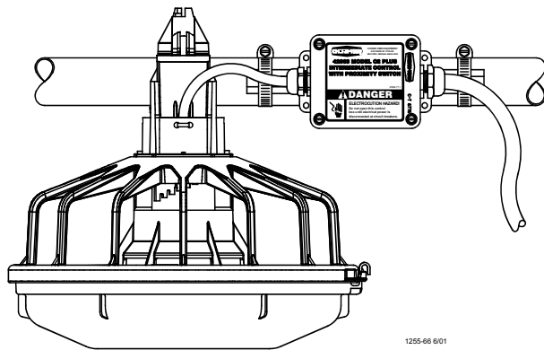
MODEL C2 PLUS Mid-Line Control with (ES) Proximity Switch
