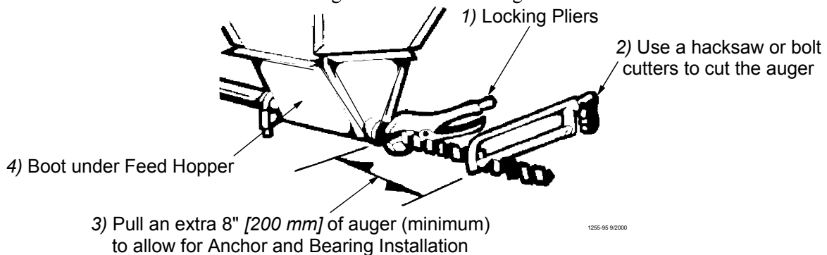
Figure 44. Cut the Auger with required stretch
