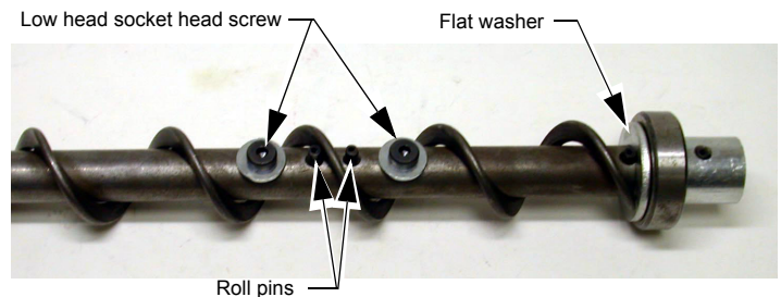
Figure 61. Auger and Anchor Bearing Connection
