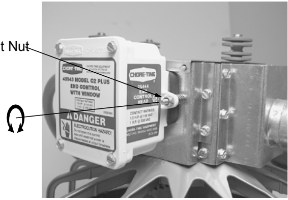
Figure 59. Switch Adjustment
