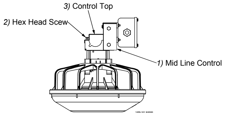
Figure 50. Mid-Line Control Installation
