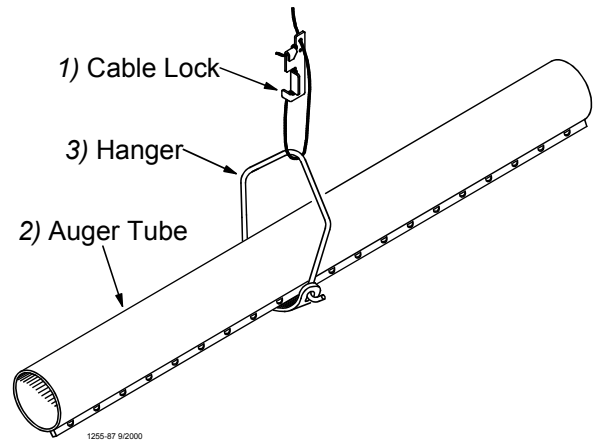
Figure 30. Hanger Installation
