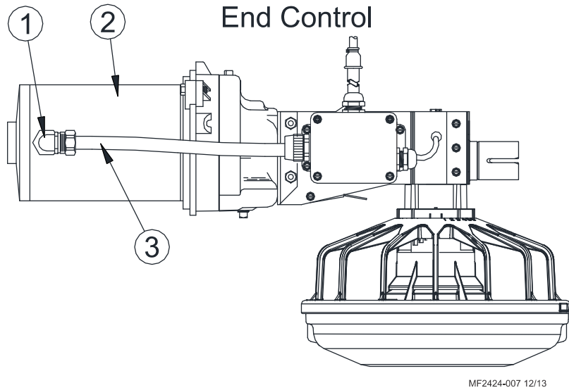
Figure 37. Installing Water Tight, Cutting and Installing Conduit
