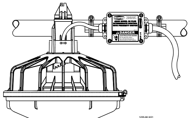
Figure 51. Installing the (ES) Mid Line Control
