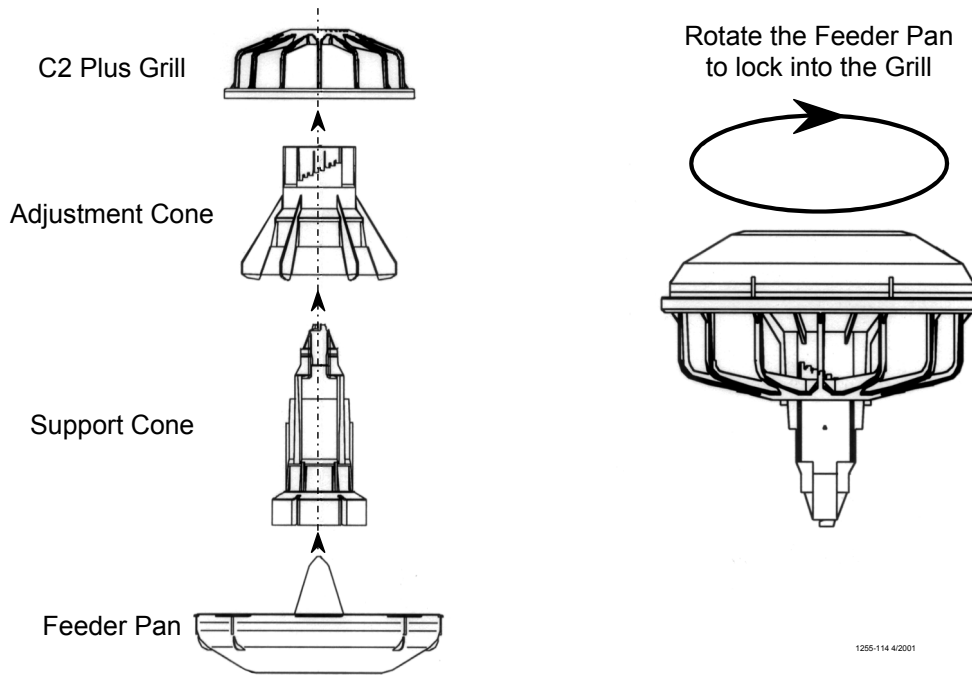
Figure 24. Assembling the Feeder Pan
