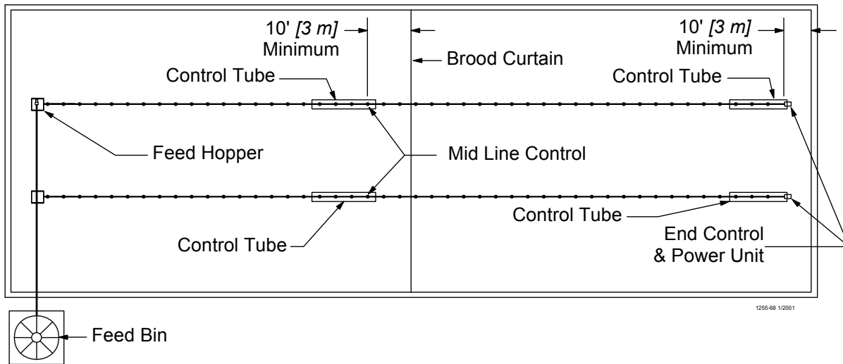
Figure 63. Component location diagram for systems over 400 feet [122 m]. (Top View).
