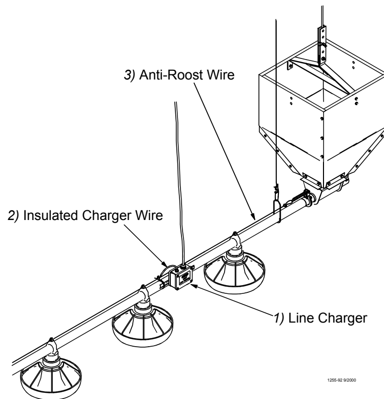
Figure 57. Line Charger Installation
