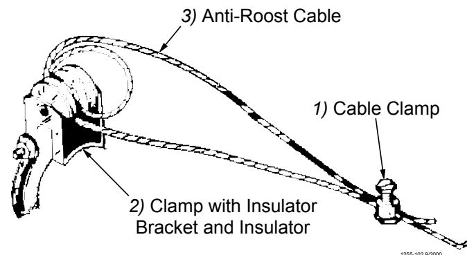
1255-102 9/2000 Figure 53. Anti-Roost Cable at the Hopper
