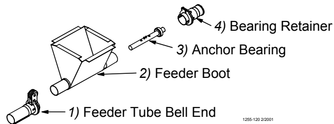
Figure 33. Installing the Feeder Boot
