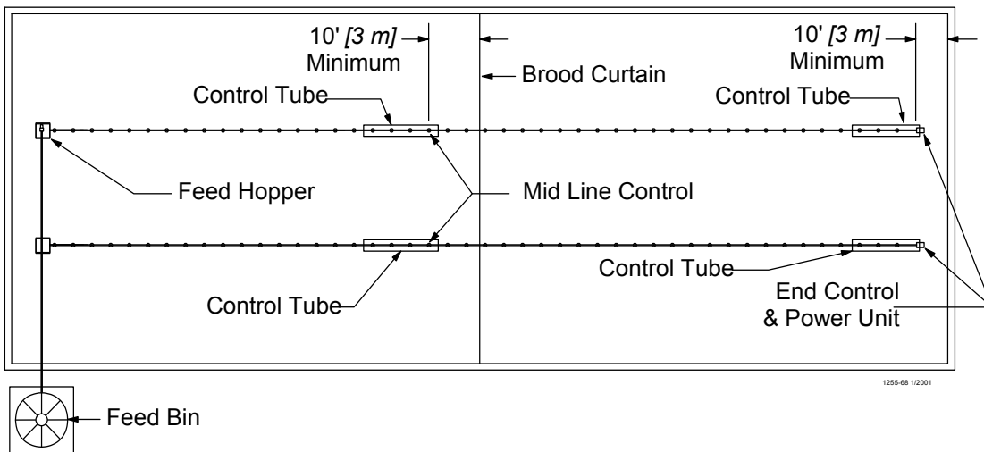
Figure 64. Component location diagram for systems up to 400 feet [122 m]. (Top View).
