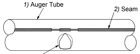
Figure 48. Mid-Line Control Location Diagram
