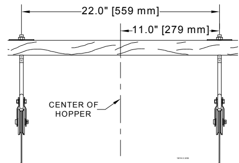
Figure 8. Steel Hopper Suspension
