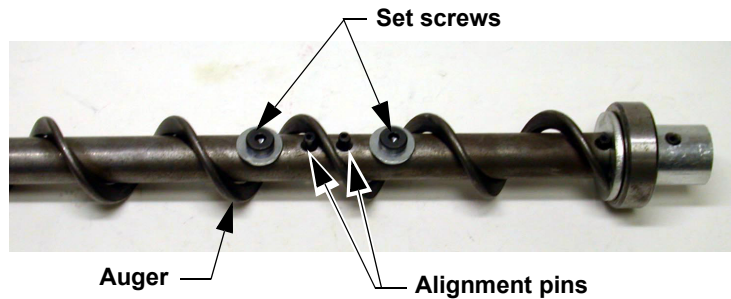
Figure 45. Auger and Anchor Bearing Connection
