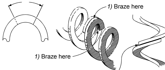
Figure 46. Auger Brazing
