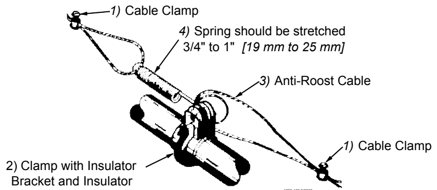
1255-103 9/2000 Figure 54. Anti-Roost Cable Mid-Line Connection
