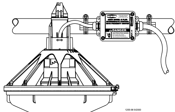
MODEL G PLUS Mid-Line Control with (ES) Proximity Switch
