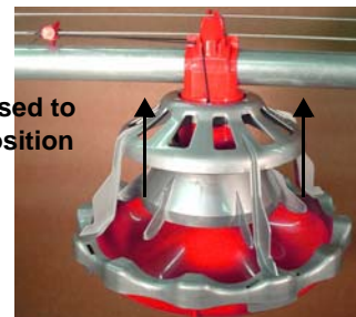
Figure 2. Actuator Winch Setting # 3
