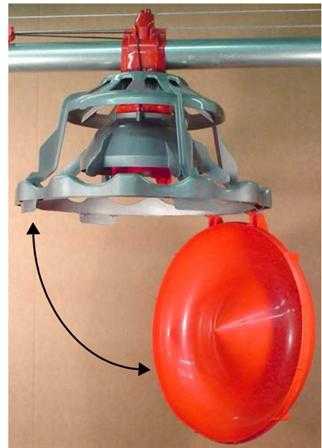
Figure 6. Swing Pan Down for Cleaning
