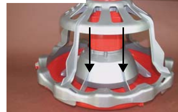
Figure 5. Rotate and Lower Cone
