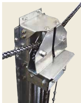
Chain-Sprocket Model
